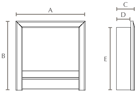
A) Width 614mm | B) Height 611mm | C) Depth 170mm D) Inset 135mm | E) Rear Height 565mm
